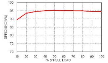
DOS16-05T, Vout=3.3V Efficiency vs. Output Load
