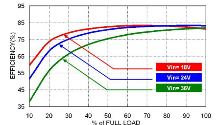
EDL02-24S05 Efficiency vs. Output Load
