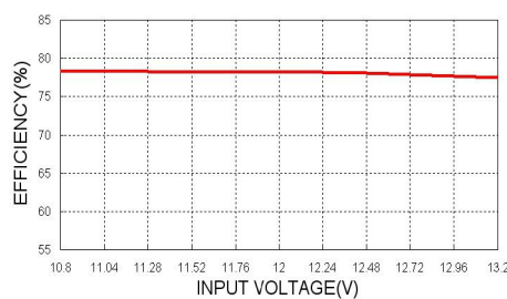
DU1P0-12S05 Efficiency vs. Input Voltage
