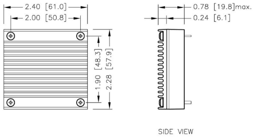
HAE200-□□S□□W -HS4 7GA0127P01-F
