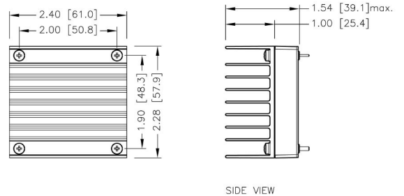
HAE200-□□S□□W -HS5 7GA0128P01-F
