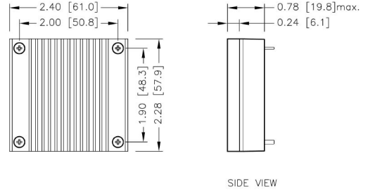
HAE200-□□S□□W -HS1 7G-0022A-F
