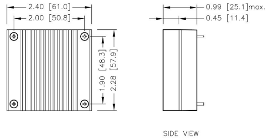
HAE200-□□S□□W -HS5 7GA0128P01-F
