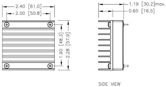
HAE200-□□S□□W -HS4 7GA0127P01-F
