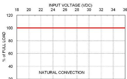
PDL09-24S12M Load Derating v.s. Input Voltage (at Ta=60°C)
