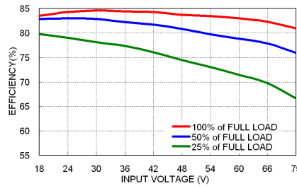
MPP03-48S05WA Efficiency vs. Input Voltage
